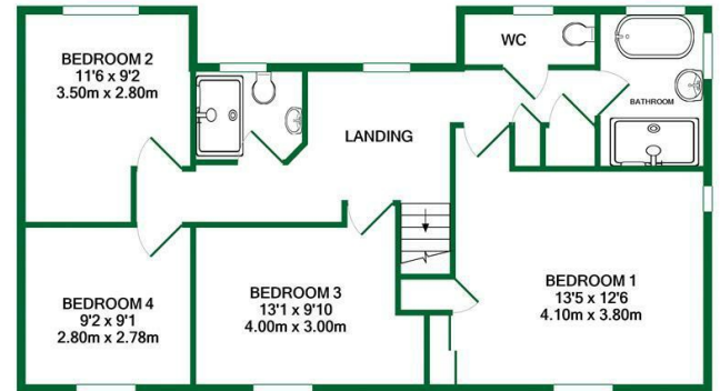
1ST FLOOR
